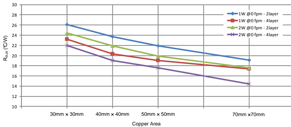
Figure 76. Measured R_{\theta JA} vs PCB Copper Area on 2-Layer Boards and 4-Layer Boards
