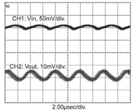
7812SR V_{in} = 24\text{V} , I_{LOAD} = 40\text{mA}
