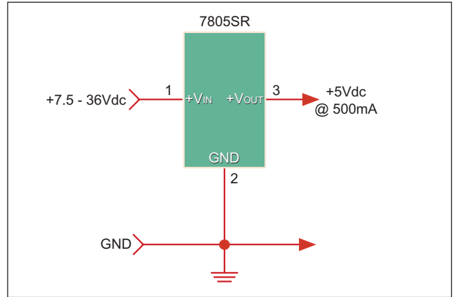
Figure 1. Typical Connections
