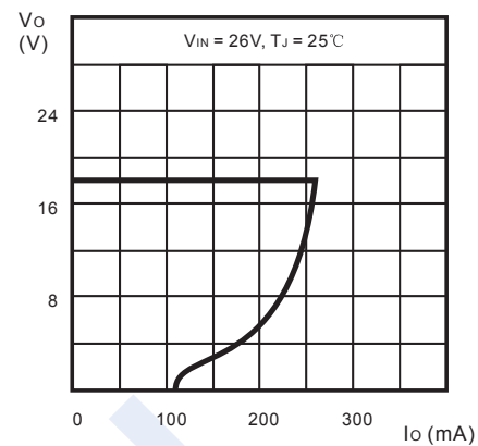
Load Characteristics
