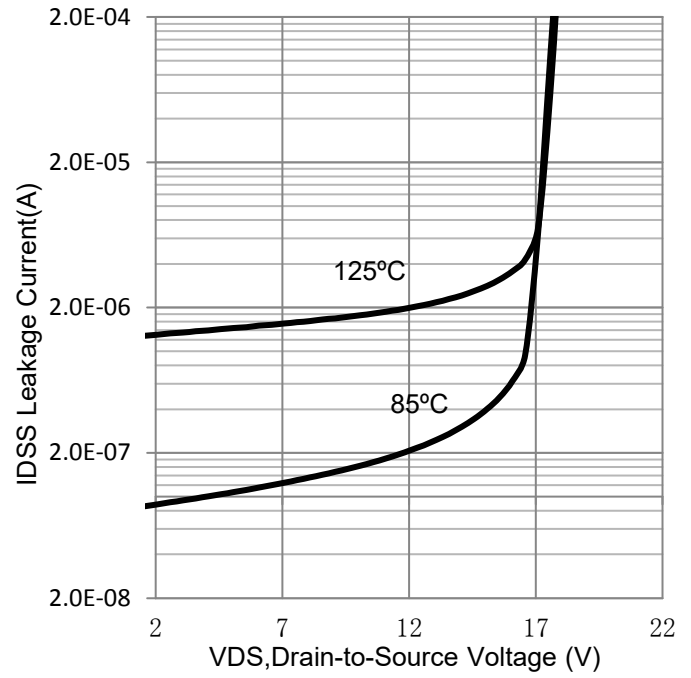
Drain-to-Source Leakage Current vs. Voltage
