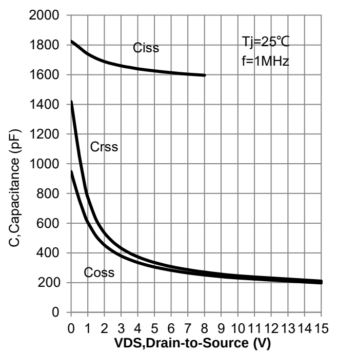
Capacitance variation
