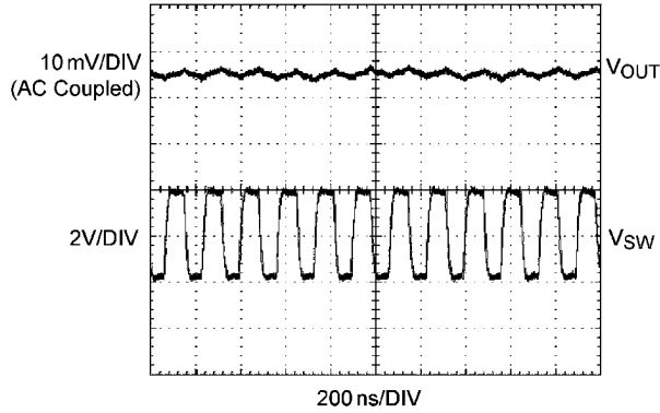
www.DataSheet4U.com Typical Switching Waveform (PWM Mode, I_{OUT} = 300\text{ mA} )
