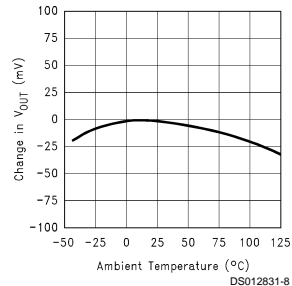
Normalized Output Voltage vs Temperature
