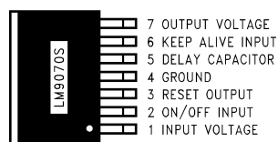
7-Lead TO-263 Surface Mount Package
