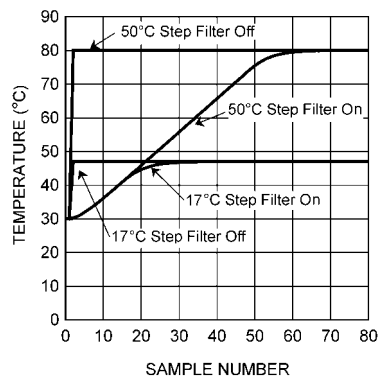
a) Seventeen and fifty degree step response 30006125
