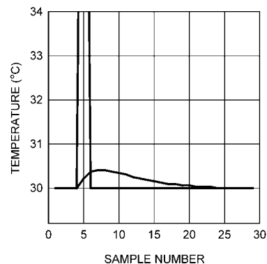
c) Impulse response with input transients greater than 4°C 30006127
