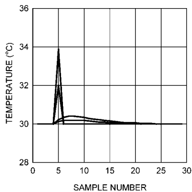
b) Impulse response with input transients less than 4°C 30006126
