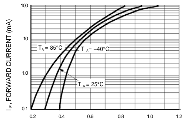
Figure 4. Forward Voltage
