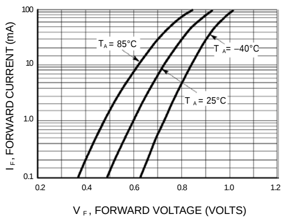
Figure 2. Forward Voltage
