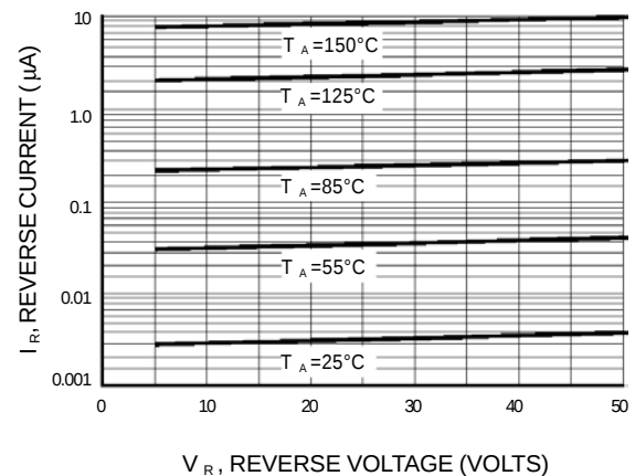
Figure 3. Leakage Current
