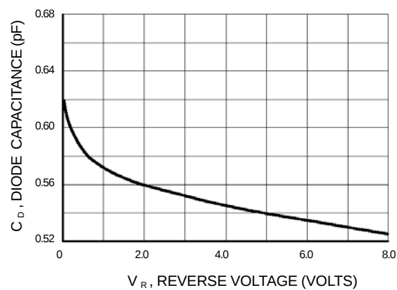
Figure 4. Capacitance
