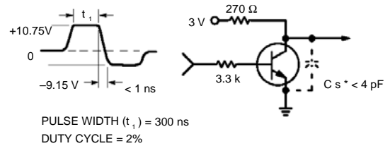
Figure 3. t_{off} Circuit — 10 mA
