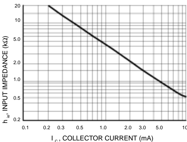
Figure 11. Input Impedance
