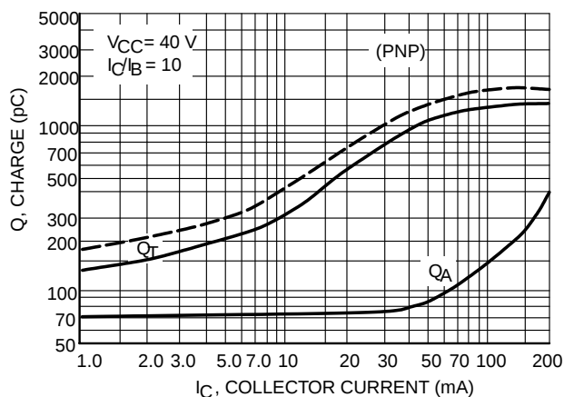
Figure 22. Charge Data
