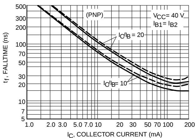
Figure 24. Fall Time
