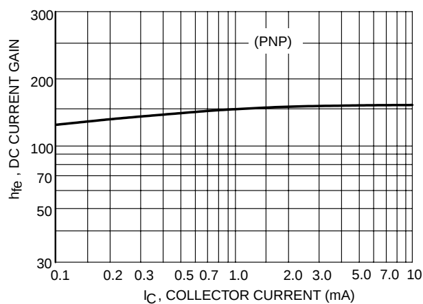
Figure 27. Current Gain
