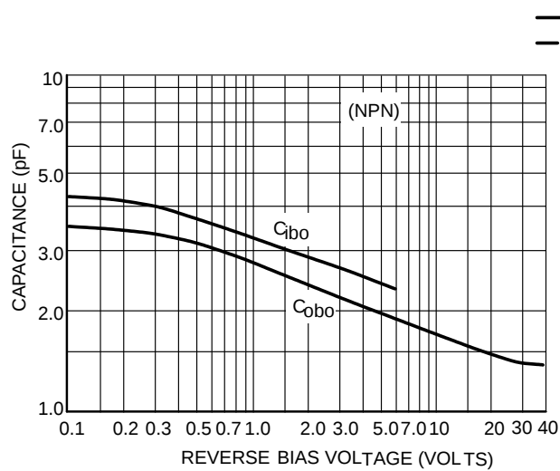
Figure 3. Capacitance
