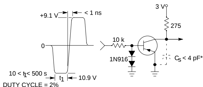
Figure 20. Storage and Fall Time Equivalent Test Circuit
