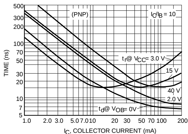
Figure 23. Turn-On Time
