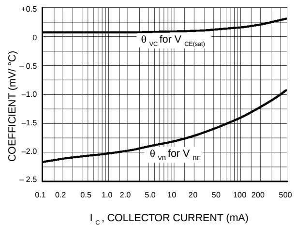
Figure 18. Temperature Coefficients
