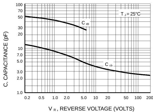
Figure 5. Capacitance
