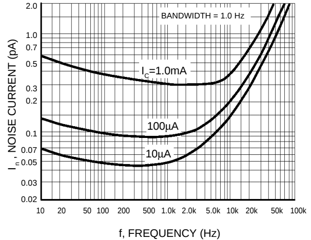
Figure 3. Noise Current
