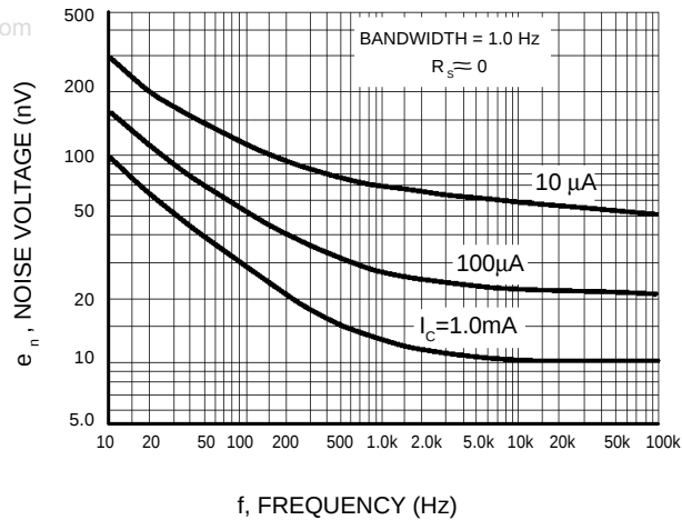
Figure 2. Noise Voltage
