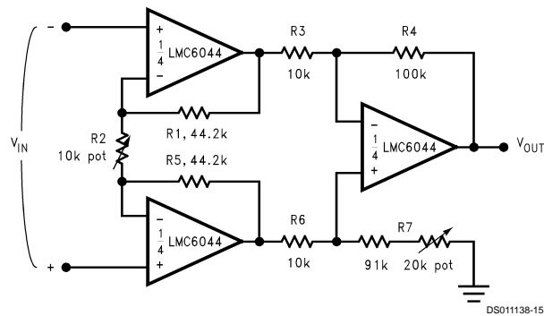
FIGURE 10. Instrumentation Amplifier
