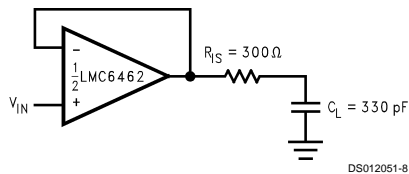
FIGURE 4. Resistive Isolation of a 300 pF Capacitive Load
