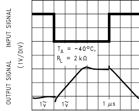
TIME (1 \mu s /DIV) DS011991-61
