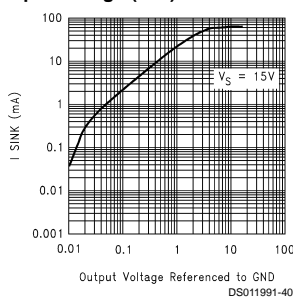
Sinking Current vs Output Voltage (15V)
