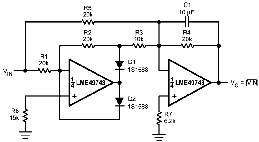
AC/DC Converter
