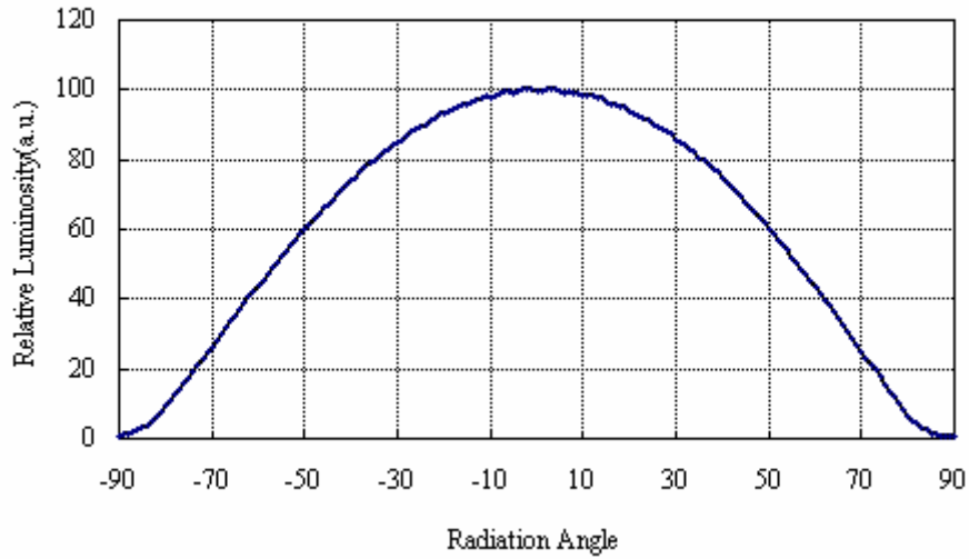
X-axis-Directivity Graph(LMFLSP100)
