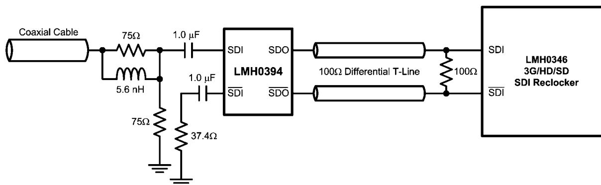
FIGURE 4. DC Output Interface to LMH0346 Reclocker
