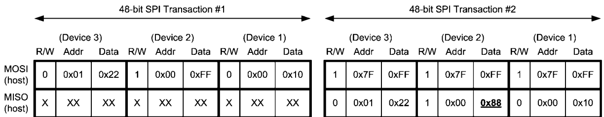
FIGURE 9. SPI Daisy-Chain Read and Write Example
