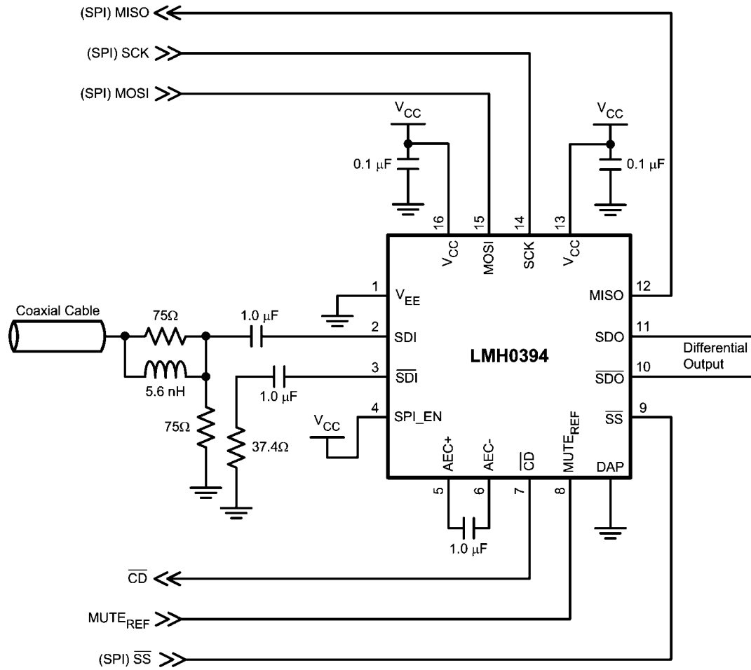
FIGURE 12. Application Circuit (SPI Mode)
