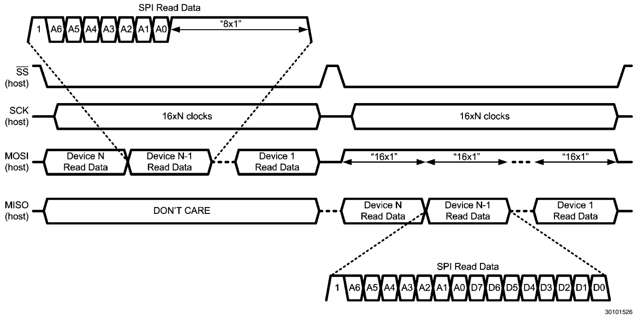
FIGURE 8. SPI Daisy-Chain Read
