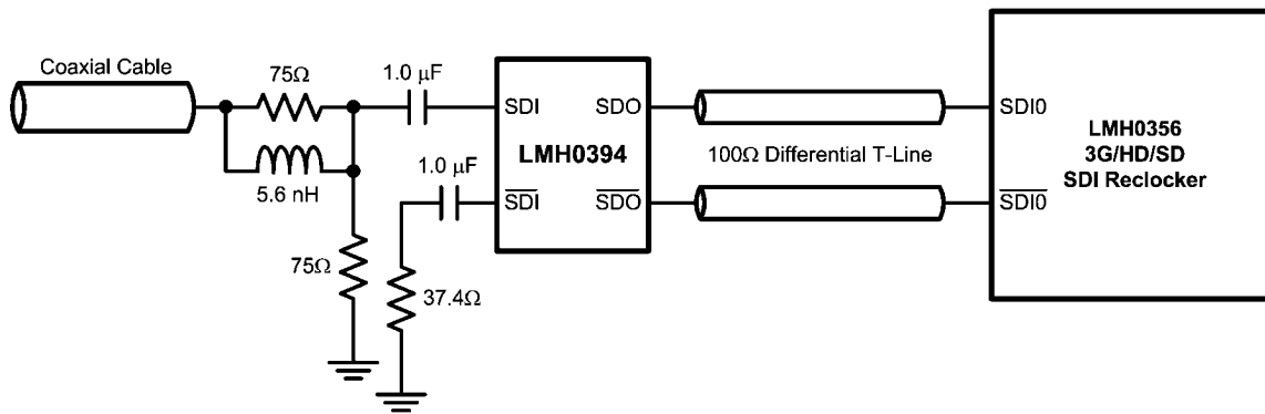
FIGURE 5. DC Output Interface to LMH0356 Reclocker
