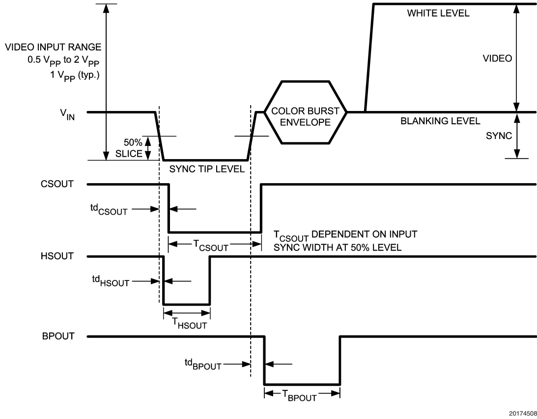
FIGURE 9. SD/EDTV Horizontal Interval with Bi-level Sync
