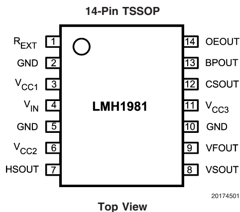
FIGURE 1. Pinout
