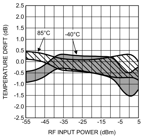
Temperature Drift Error (Mean ±3 sigma) vs. RF Input Power at 1855 MHz
