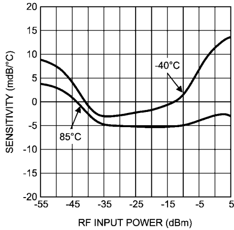
www.DataSheet4U.com Mean Temperature Sensitivity vs. RF Input Power at 50 MHz
