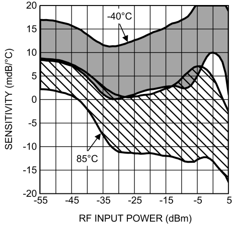
www.DataSheet4U.com Temperature Sensitivity (Mean \pm 3 sigma) vs. RF Input Power at 3500 MHz
