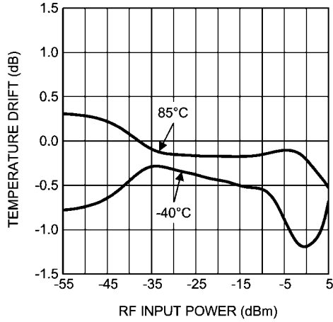
www.DataSheet4U.com Mean Temperature Drift Error vs. RF Input Power at 3000 MHz
