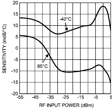
Mean Temperature Sensitivity vs. RF Input power at 4000 MHz
