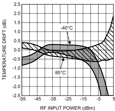
Temperature Drift Error (Mean ±3 sigma) vs. RF Input Power at 900 MHz
