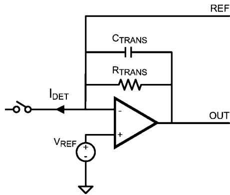
FIGURE 13. Output Stage of the LMH2100
