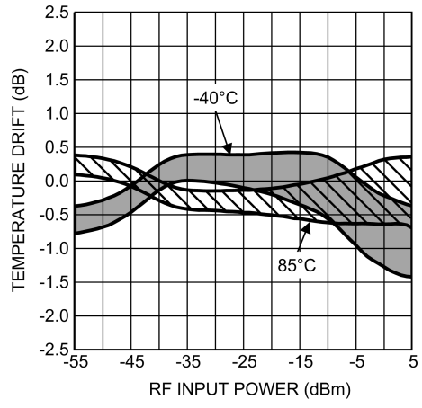
Temperature Drift Error (Mean ±3 sigma) vs. RF Input Power at 50 MHz
