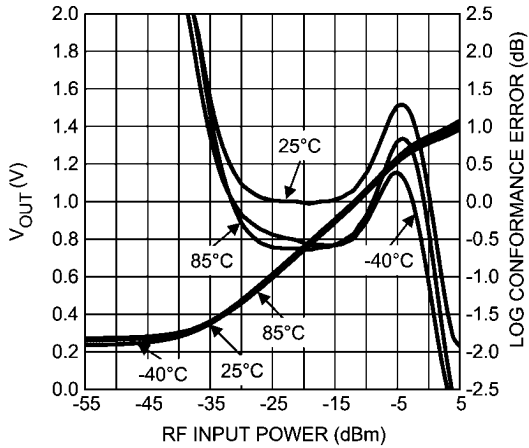
www.DataSheet4U.com Mean Output Voltage and Log Conformance Error vs. RF Input Power at 4000 MHz
