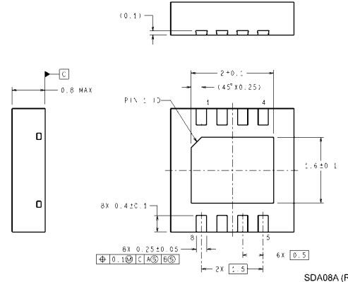
8-Pin LLP NS Package Number SDA08A
