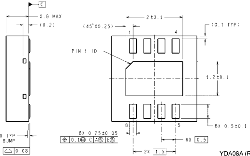
8-Pin LLP NS Package Number YDA08A
