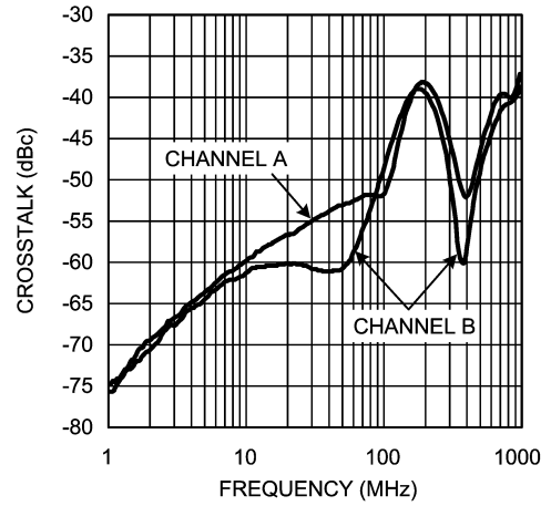
Crosstalk (LMH6724)
