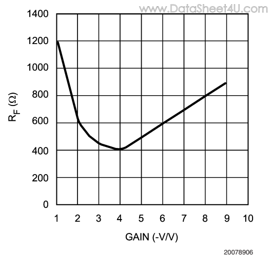
FIGURE 3. R F vs. Inverting Gain
