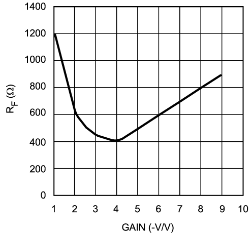
Suggested R_F vs. Gain Inverting
