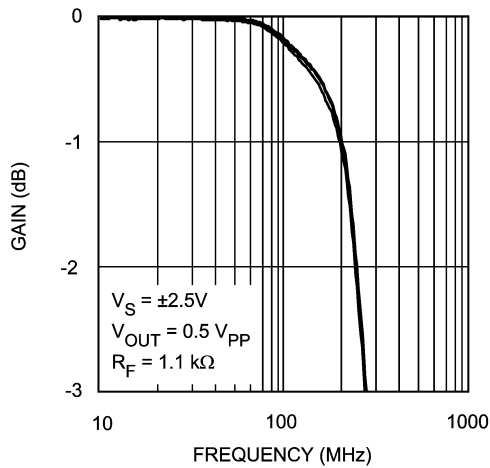
Channel Matching (LMH6725)
