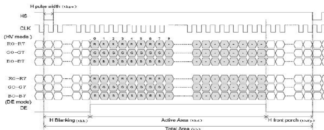
Horizontal timing
