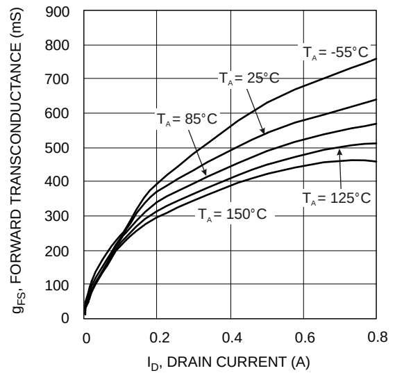
Fig. 18 Forward Transfer Conductance vs. Drain Current ( V_{DS} > I_D \cdot R_{DS(ON)} )
