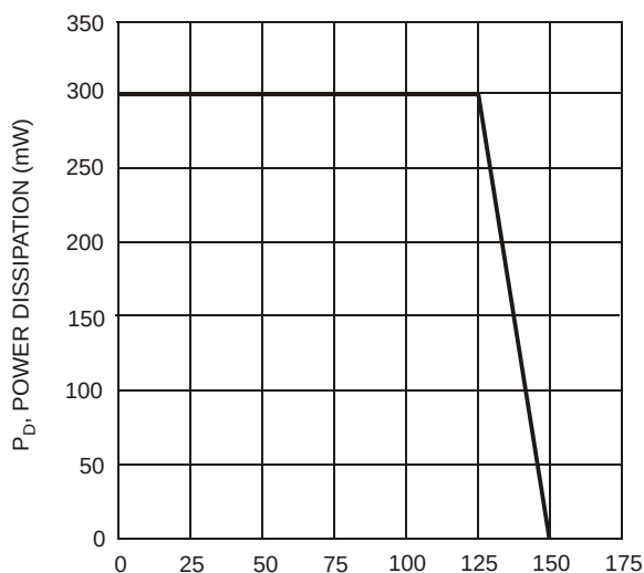
Fig. 3, Max Power Dissipation vs Ambient Temperature (Total Device)
