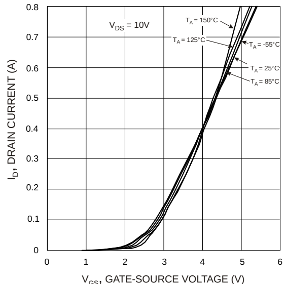
Fig. 11 Transfer Characteristics
