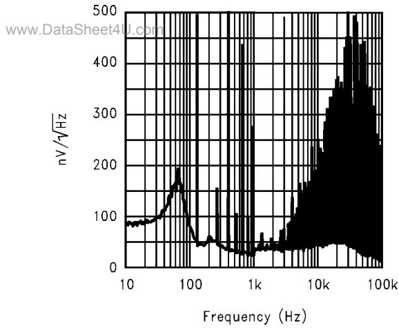
FIGURE 2. The Output of a Chopper Stabilized Op Amp (MAX432)
