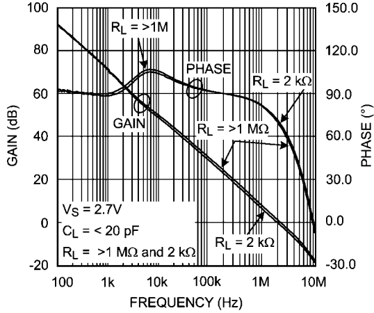
Open Loop Gain and Phase vs. Resistive Load @ 2.7V
