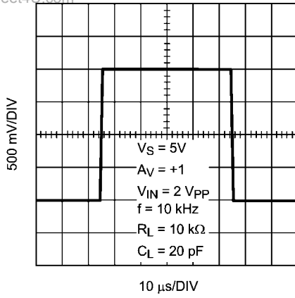
www.DataSheet4U.com Large Signal Step Response
