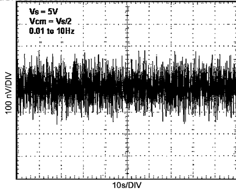
www.DataSheet4U.com Time Domain Input Voltage Noise
