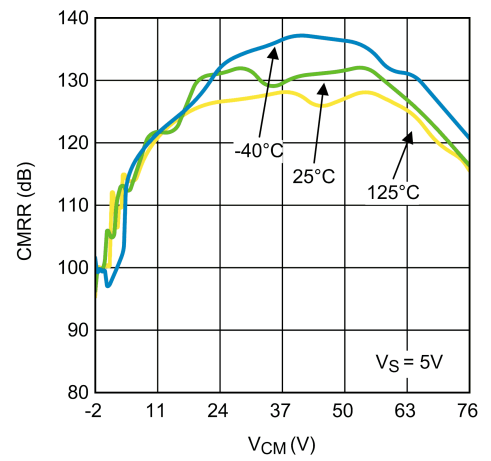
CMRR vs. V_{\text{CM}} (Gain 50V/V)
