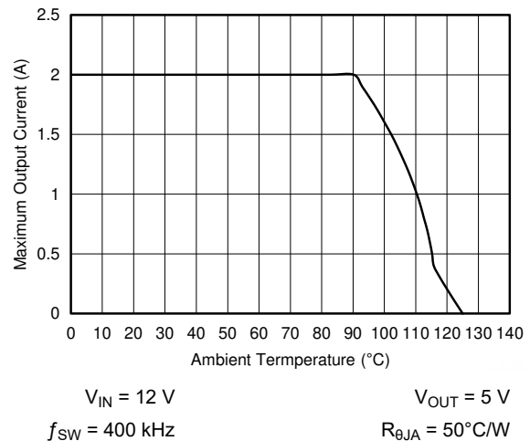
Figure 9-6. Maximum Output Current versus Ambient Temperature
