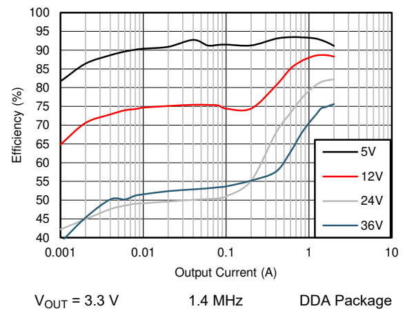
Figure 9-10. Efficiency
