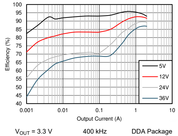
Figure 9-8. Efficiency
