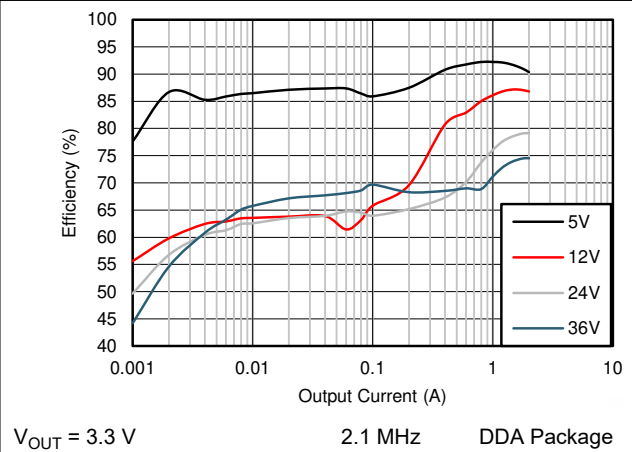
Figure 9-12. Efficiency
