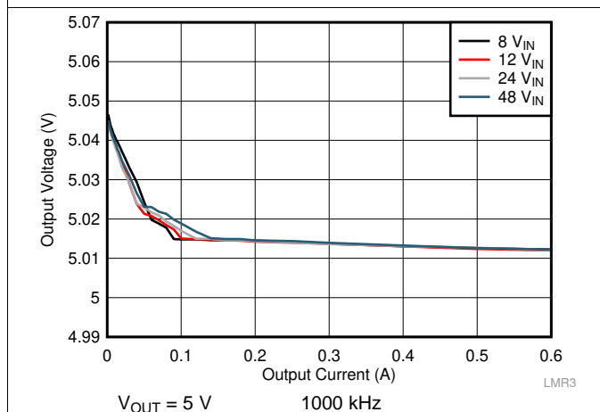
Figure 23. Load Regulation
