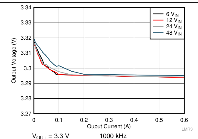
Figure 24. Load Regulation
