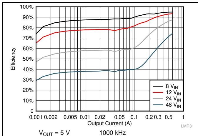
Figure 21. Efficiency
