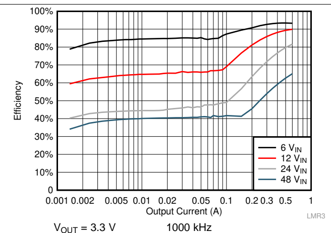
Figure 22. Efficiency
