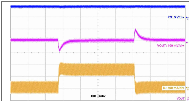
Figure 10-34. Load Transient
