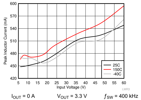
Figure 8-6. I PEAK-MIN
