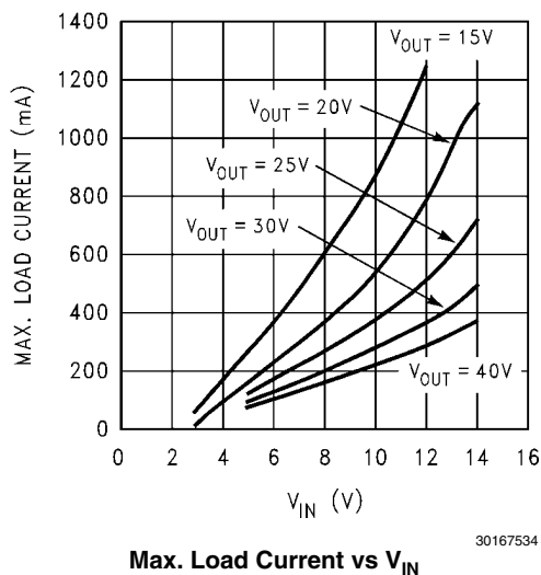
Max. Load Current vs V_{IN}
