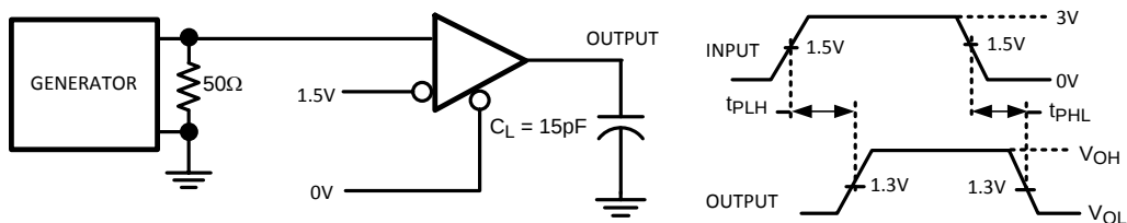
Figure 17. Test Circuit for T_{PLH} and T_{PHL}
