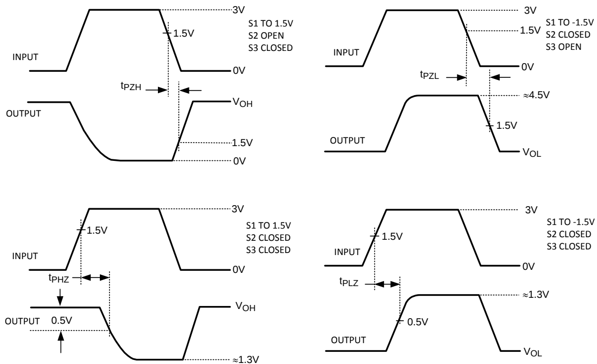
VOLTAGE WAVEFORMS
