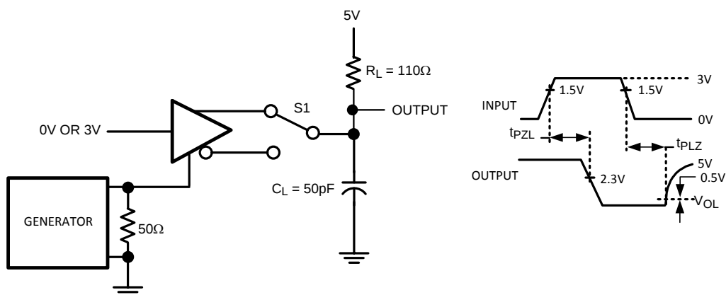
Figure 15. Test Circuit for T_{PZL} and T_{PLZ}
