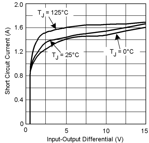
Figure 2. Short-Circuit Current
