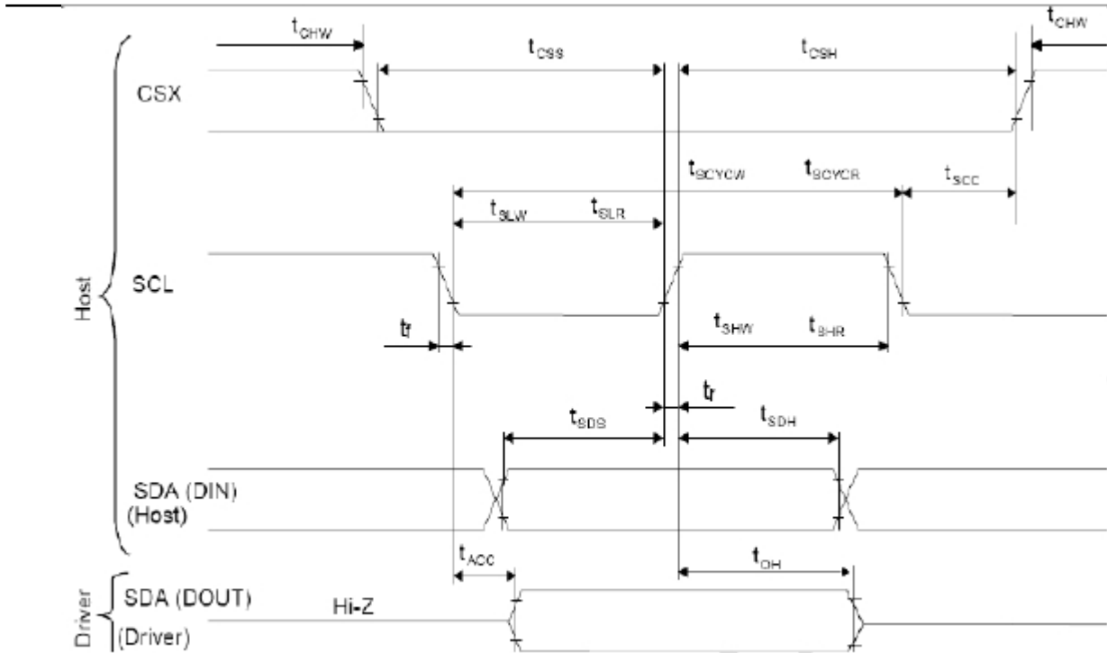
Fig.5-7 AC Characteristics of 3-Wire 9-Bit Serial Interface timing
