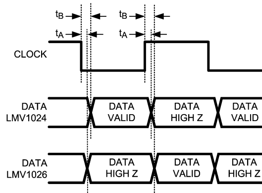
FIGURE 10. Timing
