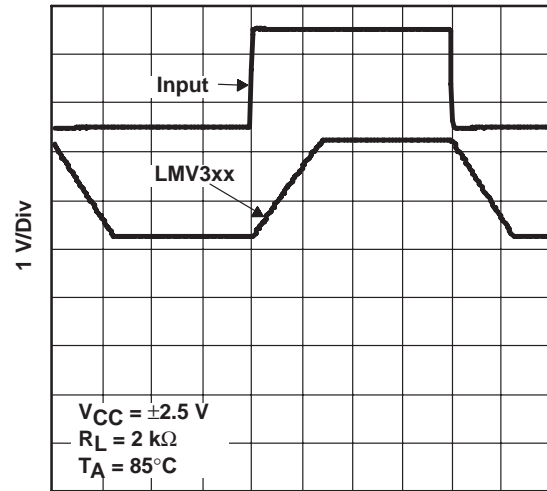
1 \mu\text{s}/\text{Div} Figure 28
