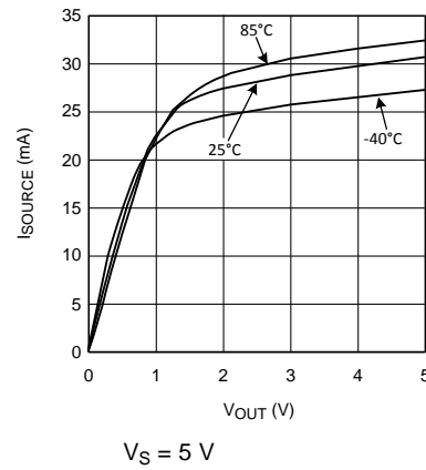
Figure 8. Sourcing Current vs Output Voltage
