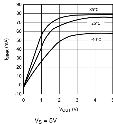
Figure 10. Sinking Current vs Output Voltage
