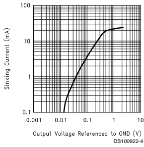
Sinking Current vs. Output Voltage ( V_S=2.2\text{V} )
