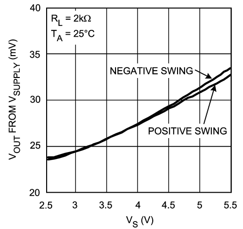
Output Swing vs. V_S
