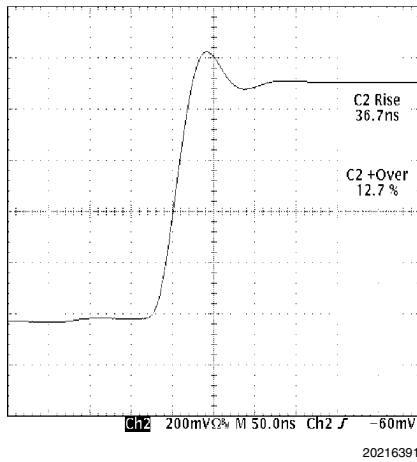
FIGURE 19. Rise Time
