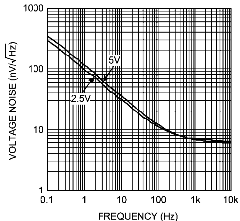
Input Referred Voltage Noise vs. Frequency 20216339
