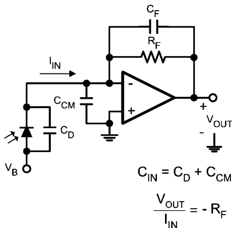
Photodiode Transimpedance Amplifier 20216369
