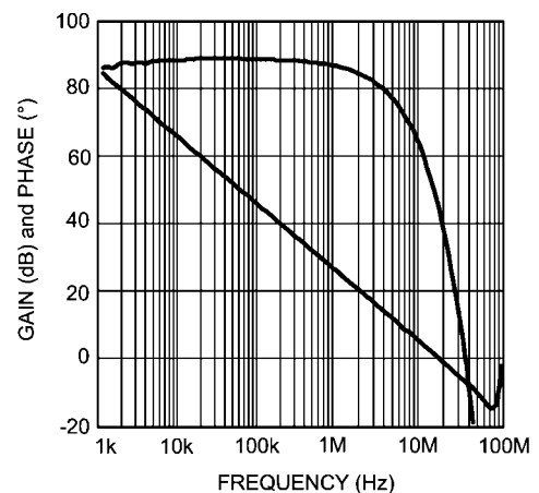
FIGURE 2. LMV796 A_{VOL} vs. Frequency
