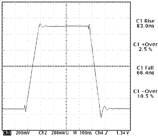
FIGURE 15. LMV796 Response Gain = +1
