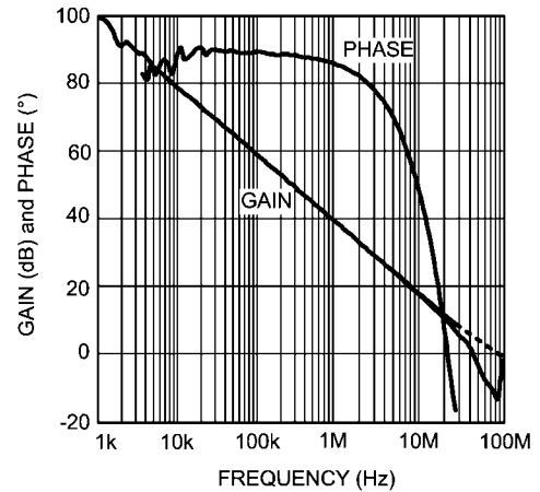
FIGURE 1. LMV793 A_{VOL} vs. Frequency
