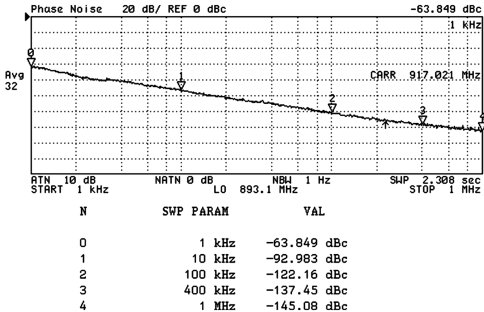
Typical phase noise characteristics in GSM band
