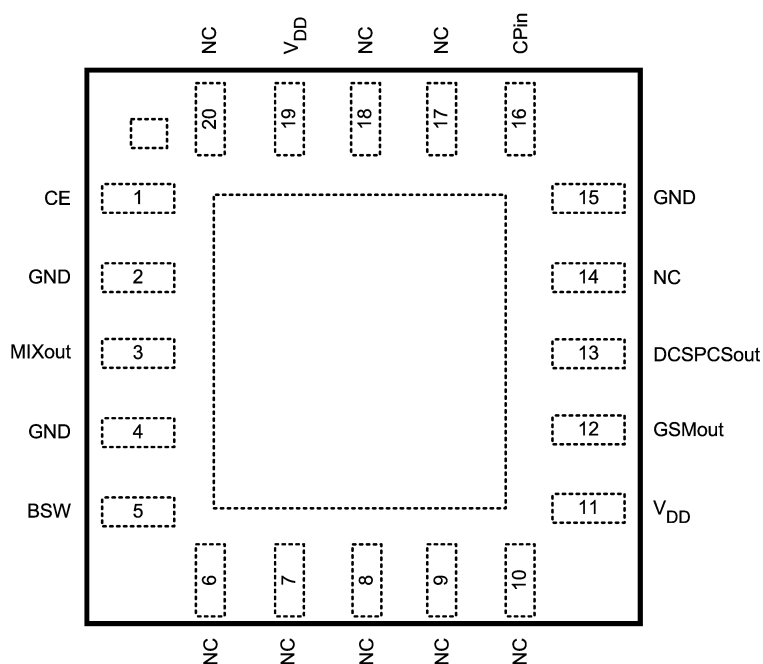
20-Pin 4x4 LLP (TM) Package
