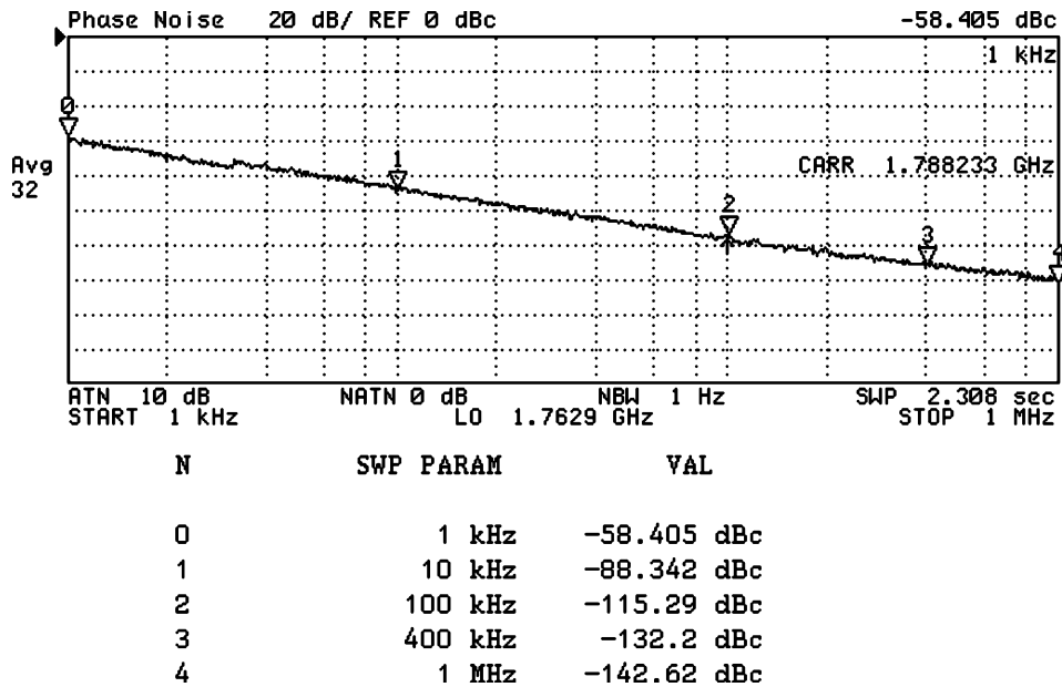
Typical phase noise characteristics in DCS band
