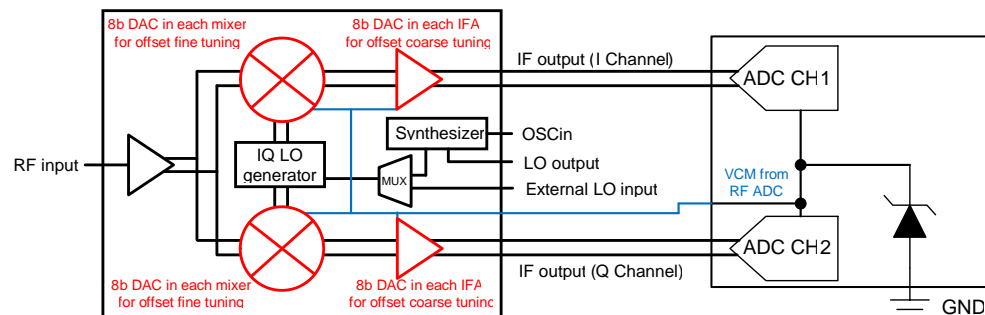
Figure 50. DC Offset Correction Diagram
