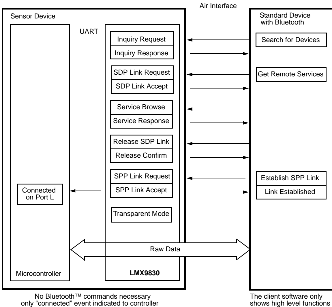
Figure 24. Point-to-Point Connection
