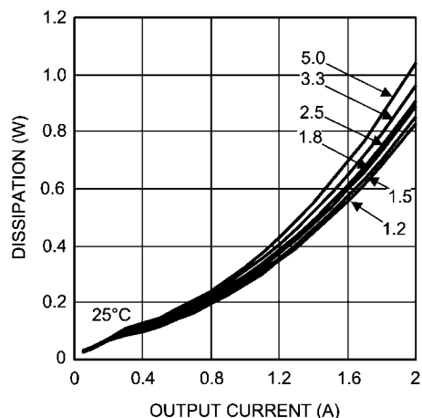
Dissipation 8V Input @ 25°C
