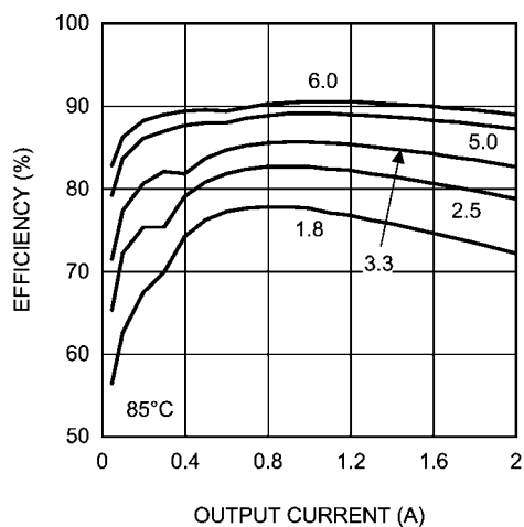
Efficiency 20V Input @ 85°C
