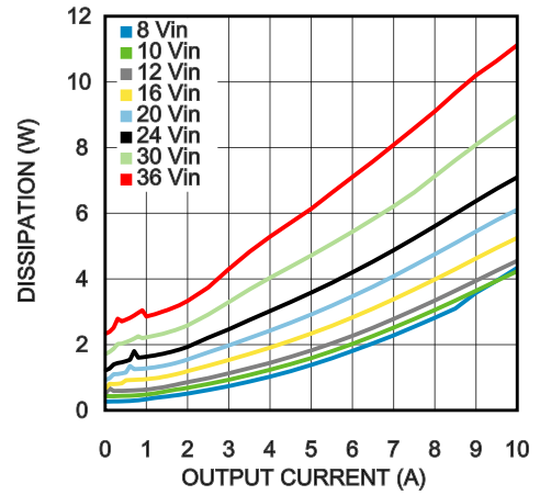
Dissipation 5.0V output @ 25^\circ C
