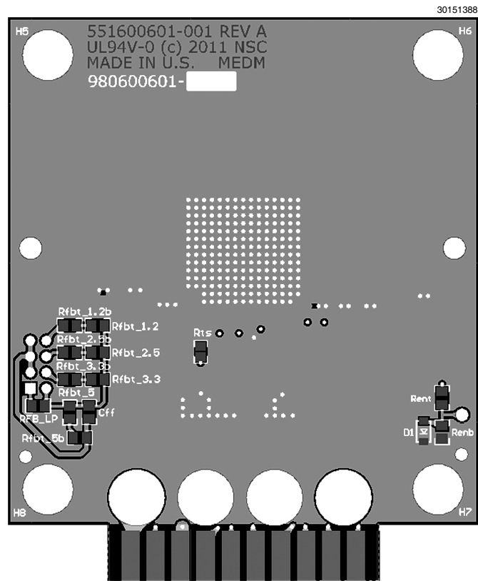
FIGURE 5. Layout Example
