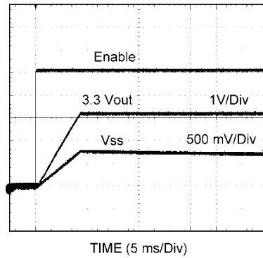
3.3V OUT Soft Start, C SS = 0.47 \mu F
