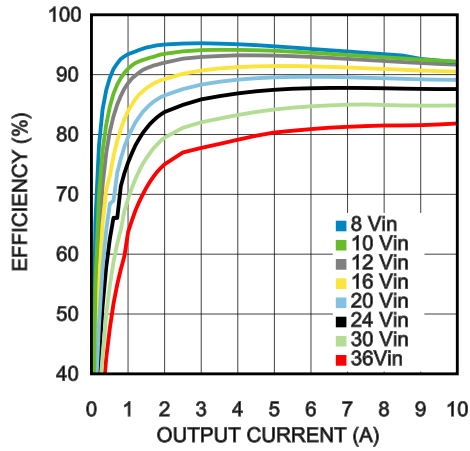
Efficiency 5.0V output @ 25^\circ C
