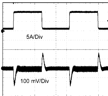
Transient response 12V IN , 5.0V OUT 1 to 10A Step
