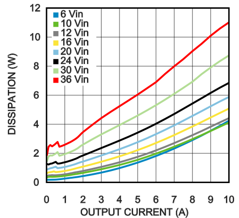
Dissipation 3.3V output @ 25^\circ C
