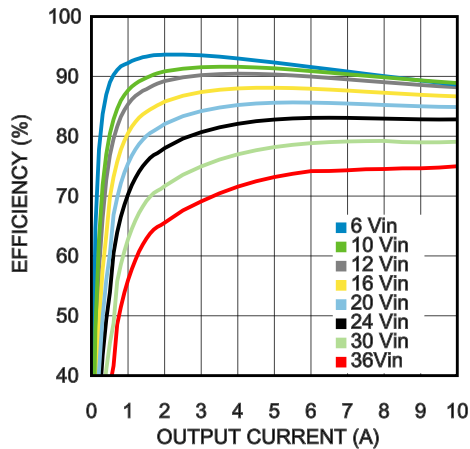
Efficiency 3.3V output @ 25^\circ C
