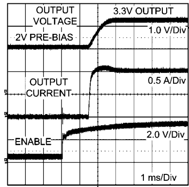
Pre-Biased Startup
